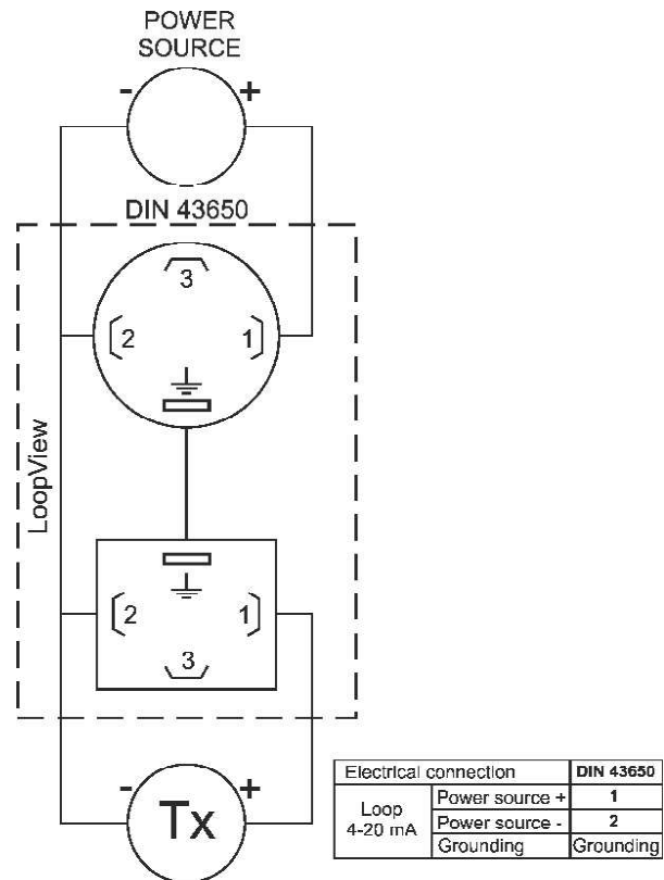
Wiring diagram
